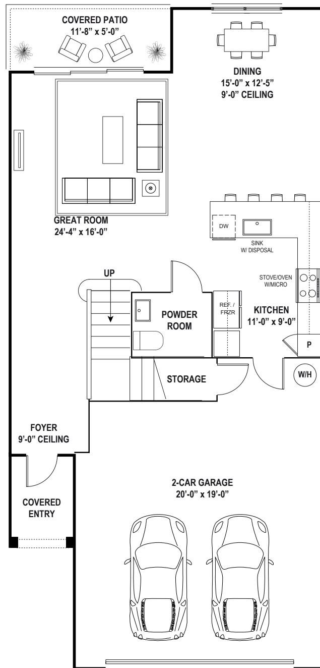
Lower Level
